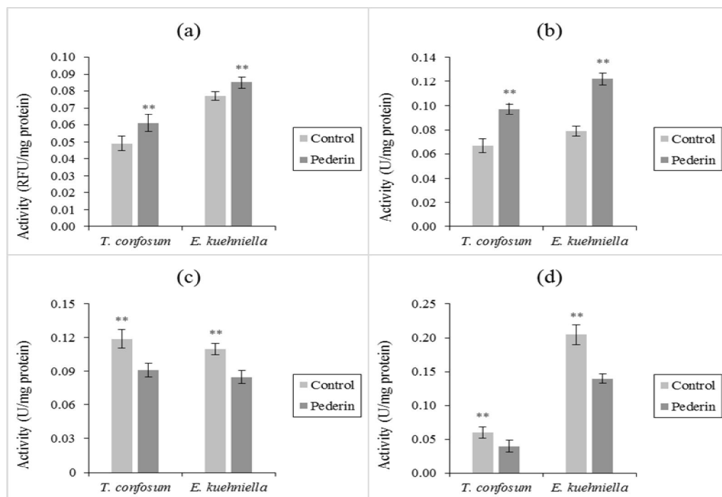
Figure 3 Activity of (a): P_{450s} monooxygenase, (b): glutathione S-transferase, and (c): carboxyl esterase and for (d): alpha and beta naphthyl acetate as substrate enzymes of Ephestia kuehniella last larval instar and Tribolium confosum adults in response to oral treatment with pederin, ** show significant difference between treatment and control at P < 0.01 (t-student test).
