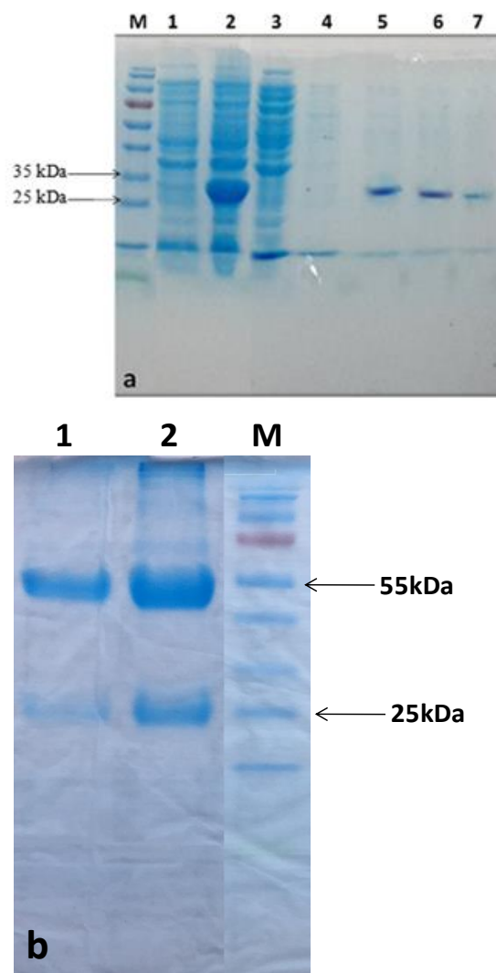
Figure 3 A: SDS-PAGE analysis of the expressed CpCDV coat protein gene in E. coli . Proteins were separated on 12% polyacrilamide gels and stained with Coomassie brilliant blue. M: pre-stained protein marker, 1: non- induced bacterial cells, 2: IPTG-induced cells, 3: flow through of column, 4: after washing, 5-7: elution steps. B: SDS-PAGE analysis of the affinity purified rabbit IgG. 1 and 2) purified IgG obtained in elution steps No. 1 and 2; M) M: pre-stained protein marker
