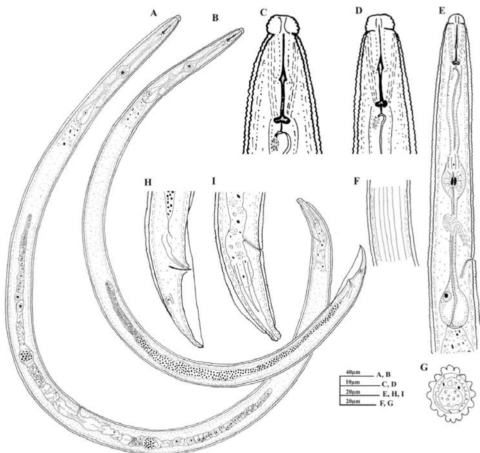
Figure 1 Iranian population of Neodolichorhynchus judithae . A: Entire female; B: Entire male; C, D: Female, head region; E: Female, anterior region; F: Female, cuticle surface; G: Female, mid-body cross section; H: Male, tail; I: Female, tail.
