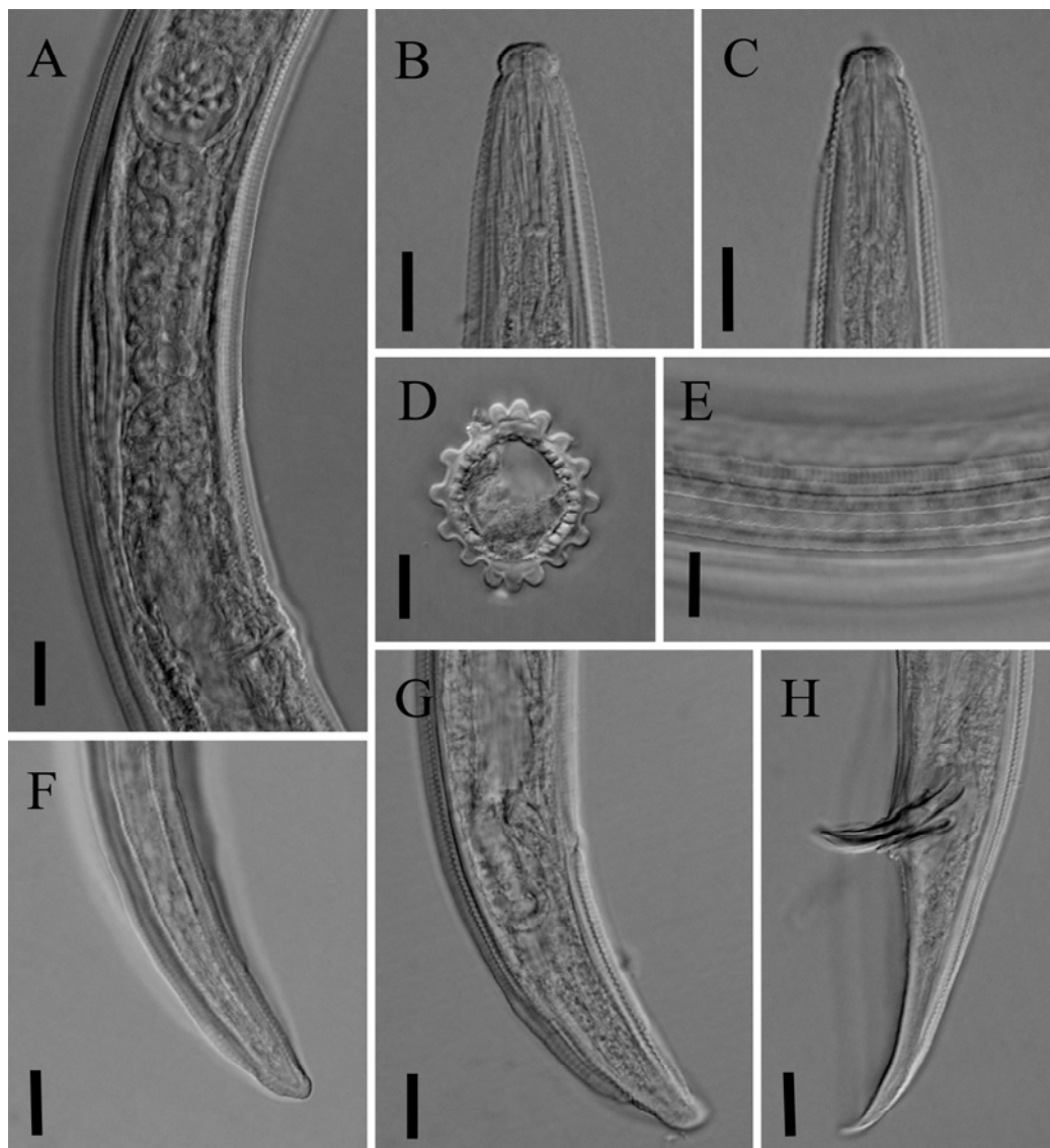
Figure 2 Iranian population of Neodolichorhynchus judthae . A: Part of female reproductive system; B & C: Female, anterior end; D: Female, mid body cross section; E: Female, longitudinal ridges; F & G: Female, tail; H: Male, cloacal region. All scale bars 10 \mu m.
