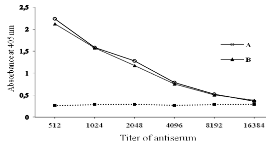
Figure 2 Titration of antiserum prepared against recombinant coat protein of cucumber mosaic virus isolate B13 by the use of indirect ELISA. The graph is based on absorbance values of the microtiter plate wells treated with different dilutions of the antiserum. A and B represent antisera of two mice as replicates. The purified protein was used as antigen.
